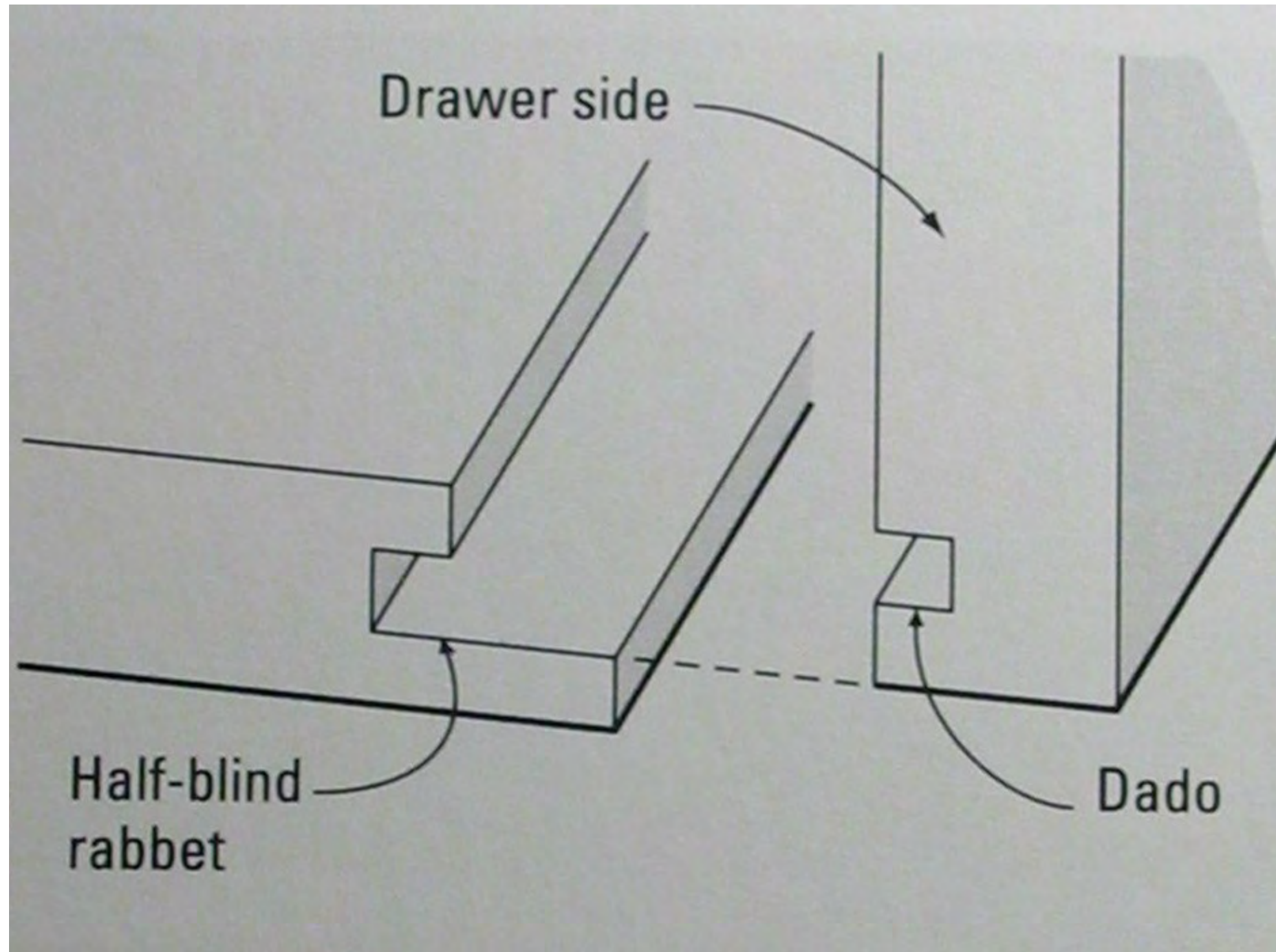
HALF-BLIND RABBET WITH DADO FOR DRAWERS
