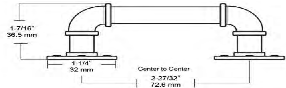
3" Industrial Pull
