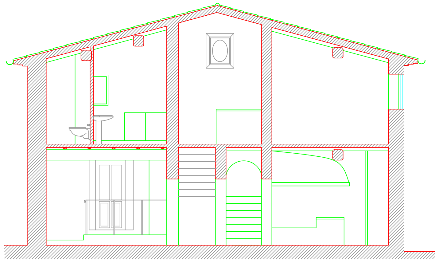
SECTION BB'
