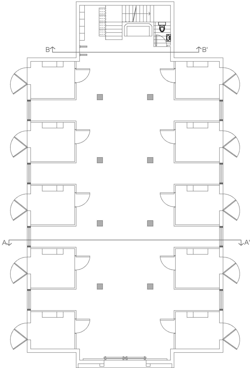
PROPOSED GA- GROUND FLOOR
